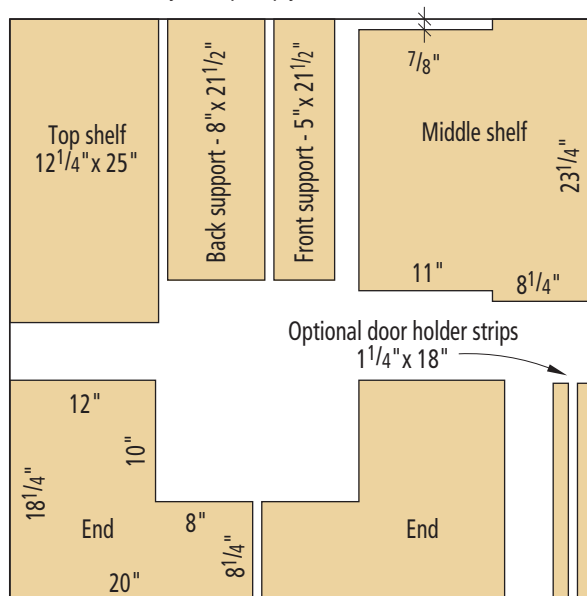
Cutting plan
