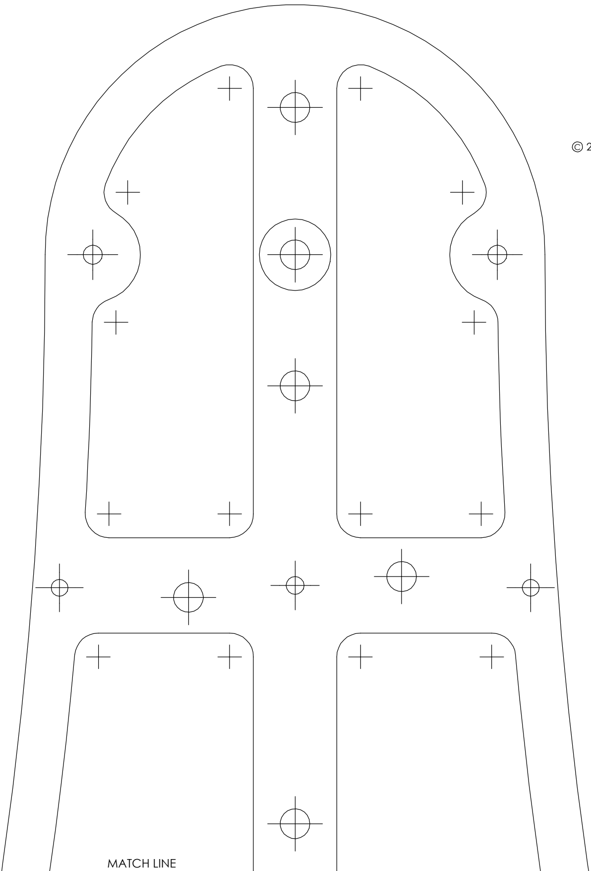
CUTTING PATTERN WC5-02-03 (TOP SECTION)
