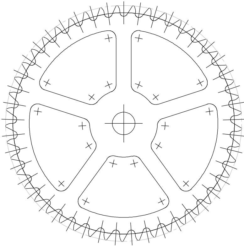
CUTTING PATTERN WC5-06-02
