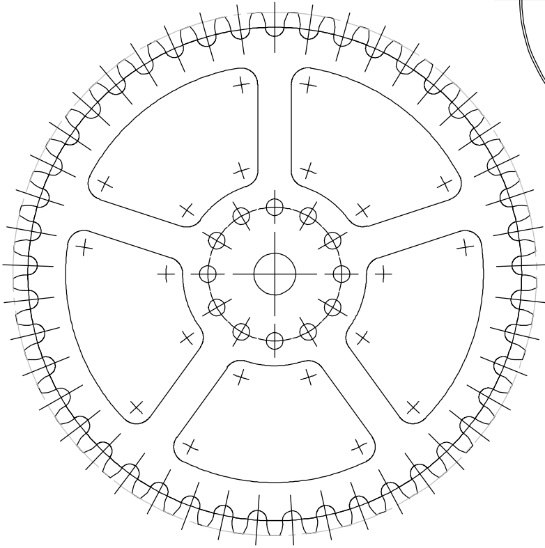
CUTTING PATTERN WC5-10-02
