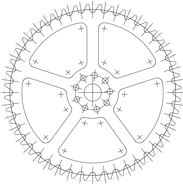
CUTTING PATTERN WC5-07-01
