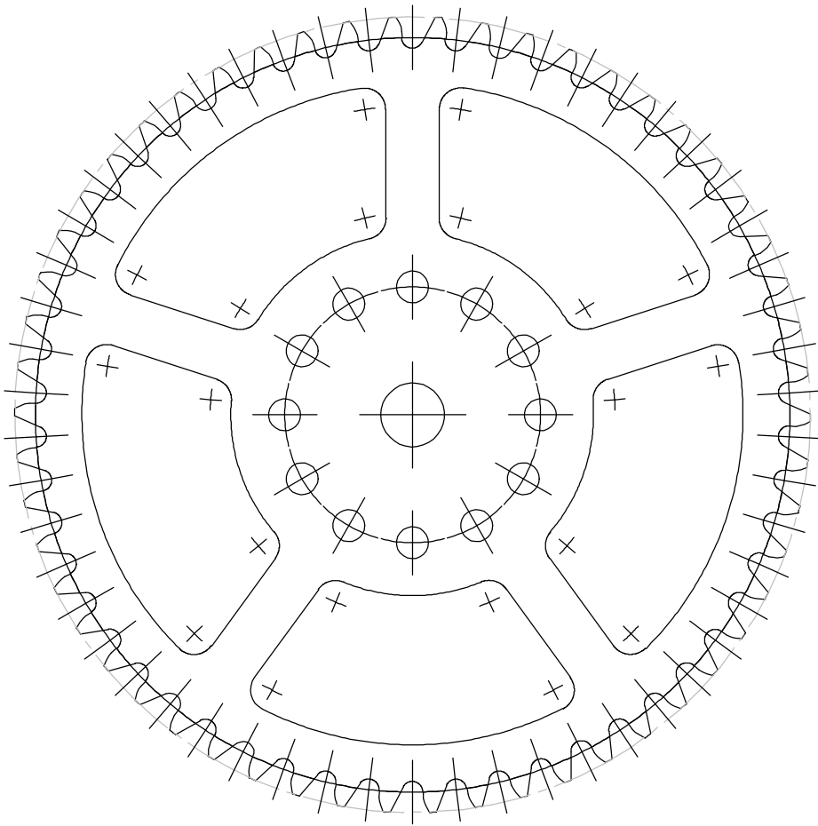
CUTTING PATTERN WC5-04-03
