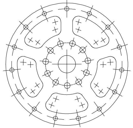
CUTTING PATTERN WC5-08-01
